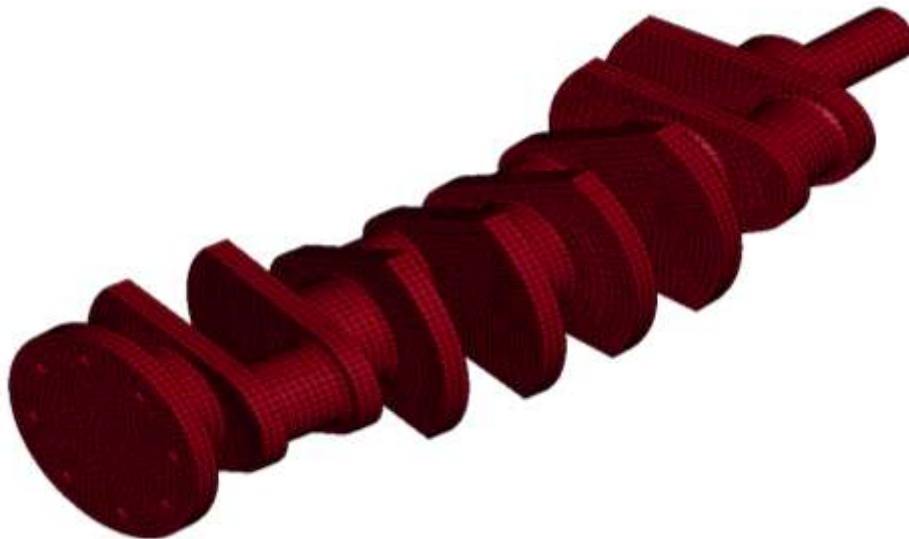
Figure 2. FEM model.
