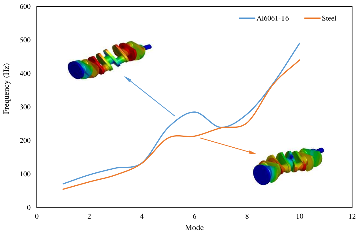
Figure 3. Frequency values depending on materials.
