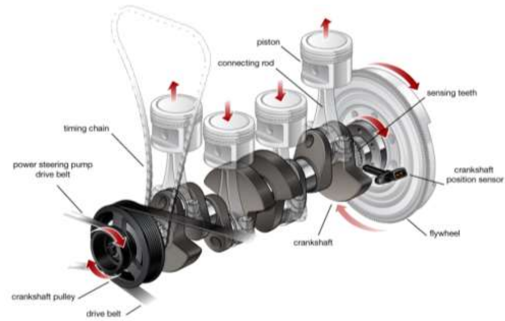
Figure 1. Loading state of the crankshaft during operation.
